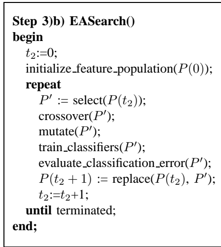
Fig. 3. Evolutionary Algorithm which replaces step 3)b) in figure 2
