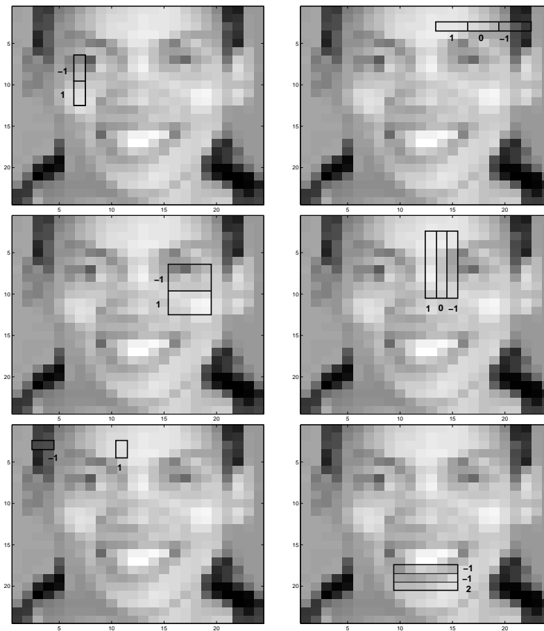
Fig. 12. First six evolved features
