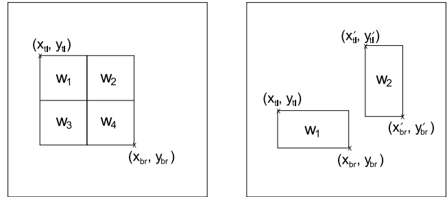
Fig. 5. Parameters for features ( k = 3 and k = 6 )
