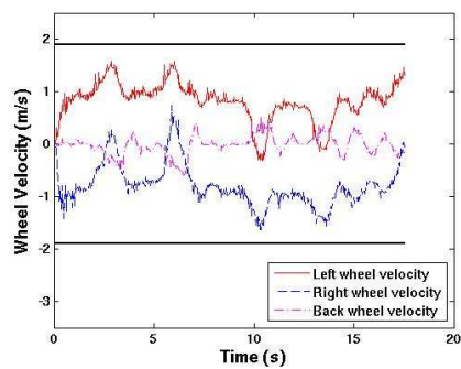
Figure 17: Real wheel velocities.
