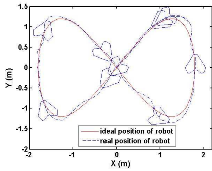
Figure 14: Reference path and robot path.
