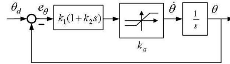
Figure 6: Closed-loop of robot orientation control.
