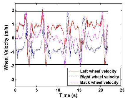
Figure 21: Real wheel velocities.
